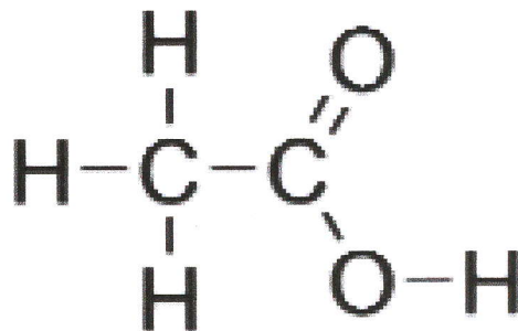
ethanoic acid
