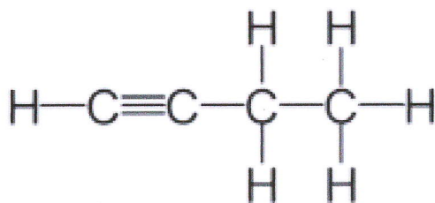
1-butyne
