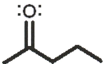
2-pentanone
