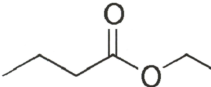
ethyl butanoate
