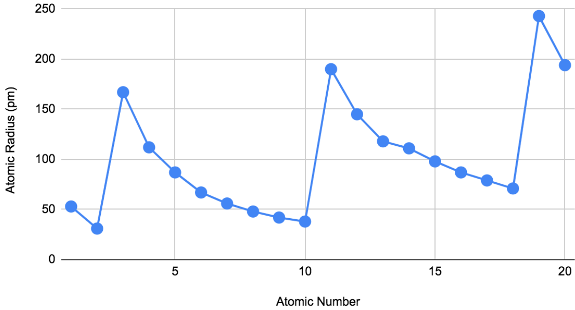
Δ Atomic Radius vs. Atomic number
